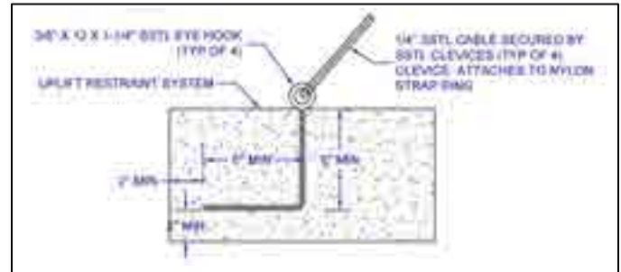
Cable tie-down detail.
