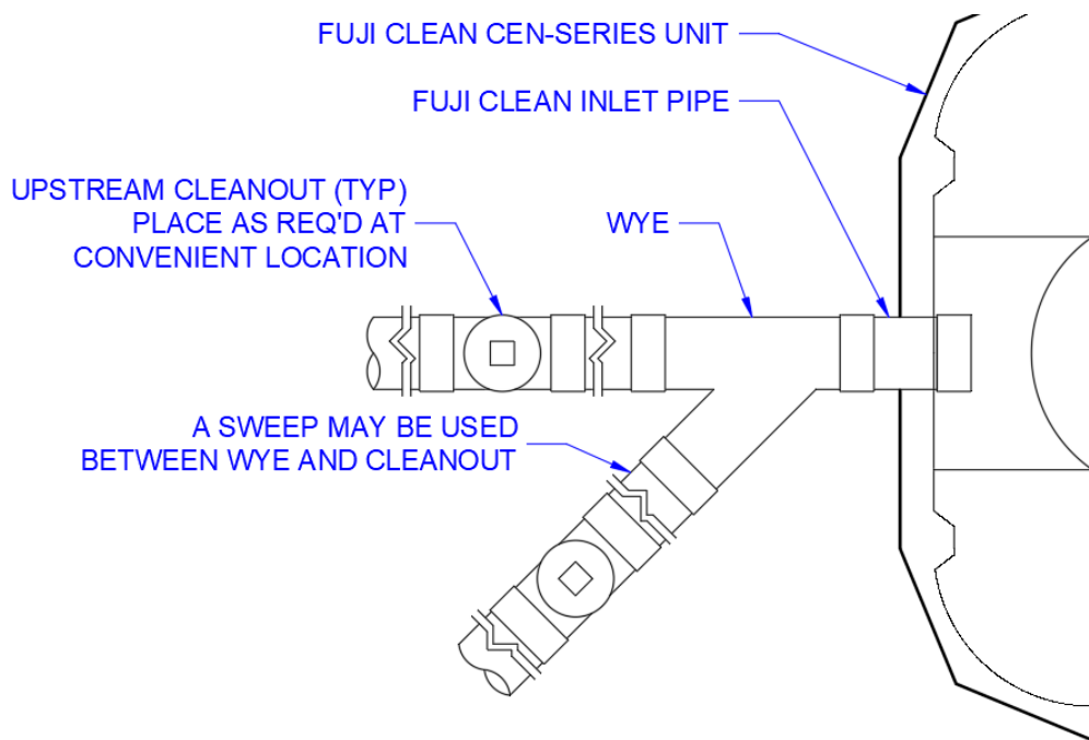
Figure 1—Inlet Laterals to Fuji Clean Unit
